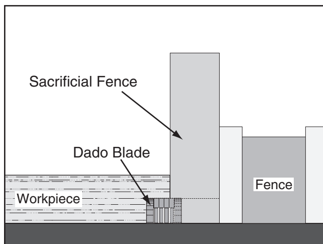
Figure 60. Rabbet cutting.
