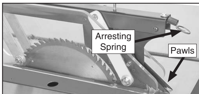
Figure 46. Pawls in resting position.
