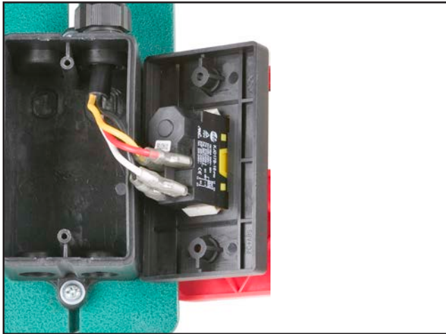
Figure 140. On/Off Switch.
