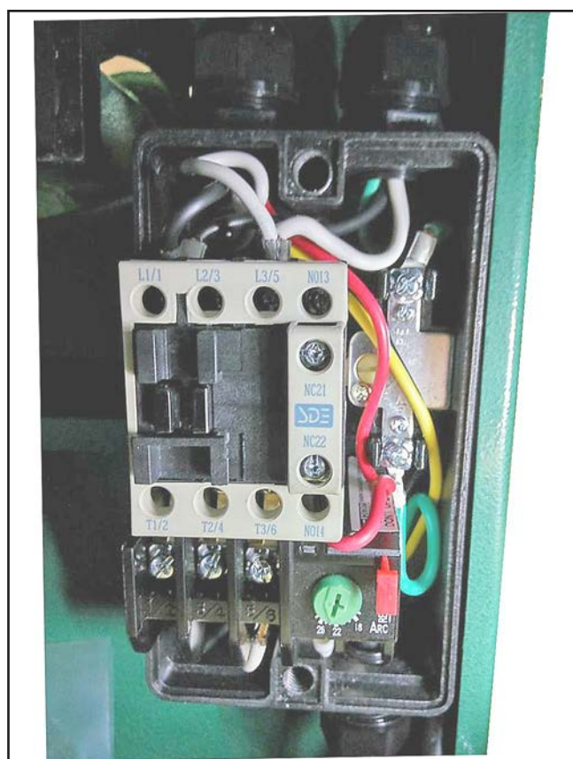
Figure 147. Magnetic switch.
