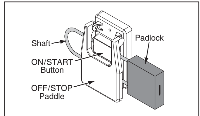
Figure 30. ON/OFF switch with disabling lock.
