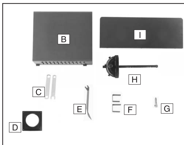
Figure 4. G1023RL main components.
