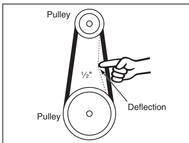
Figure 127. Checking belt tension.
