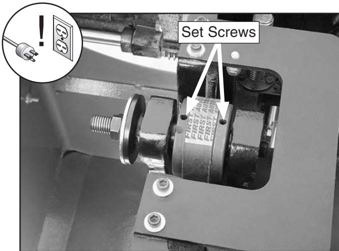
Figure 132. Location of arbor set screws.
