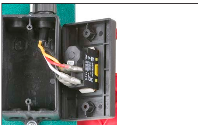
Figure 144. On/Off Switch.
