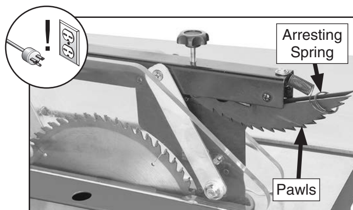
Figure 47. Pawls disabled.
